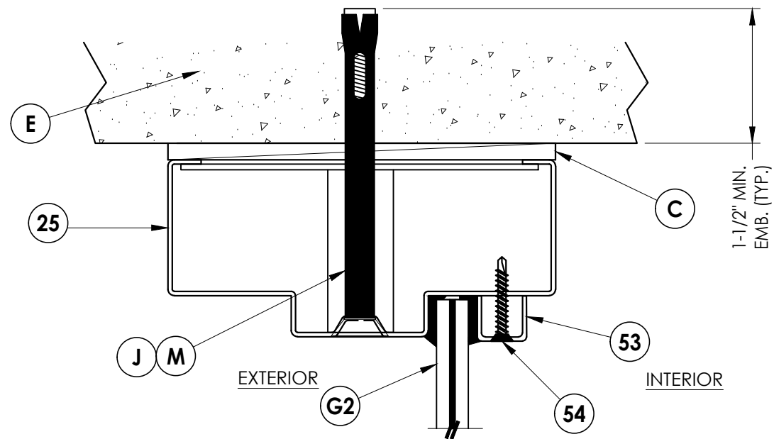
2 VERTICAL CROSS SECTION 5
